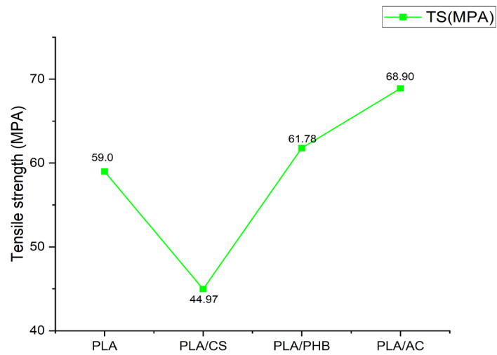
Fig. (1.a) TS for PLA and PLA bio-composite.
