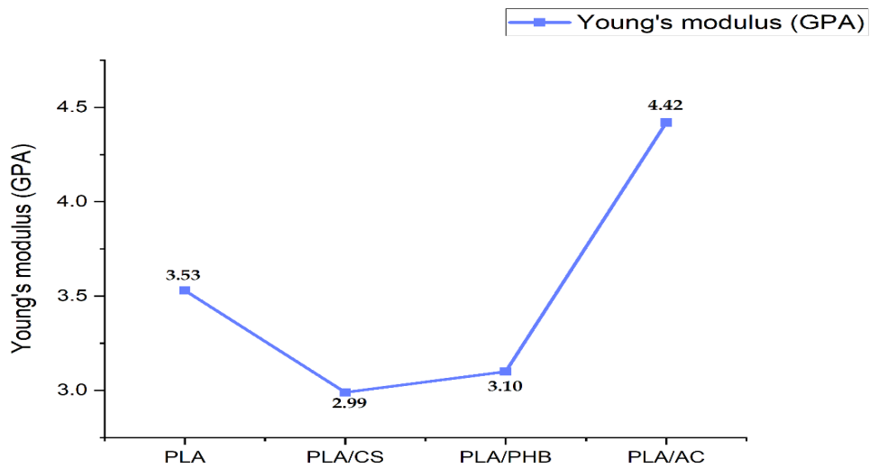
Fig. (1.b) Youngs modulus for PLA and PLA bio-composites.
