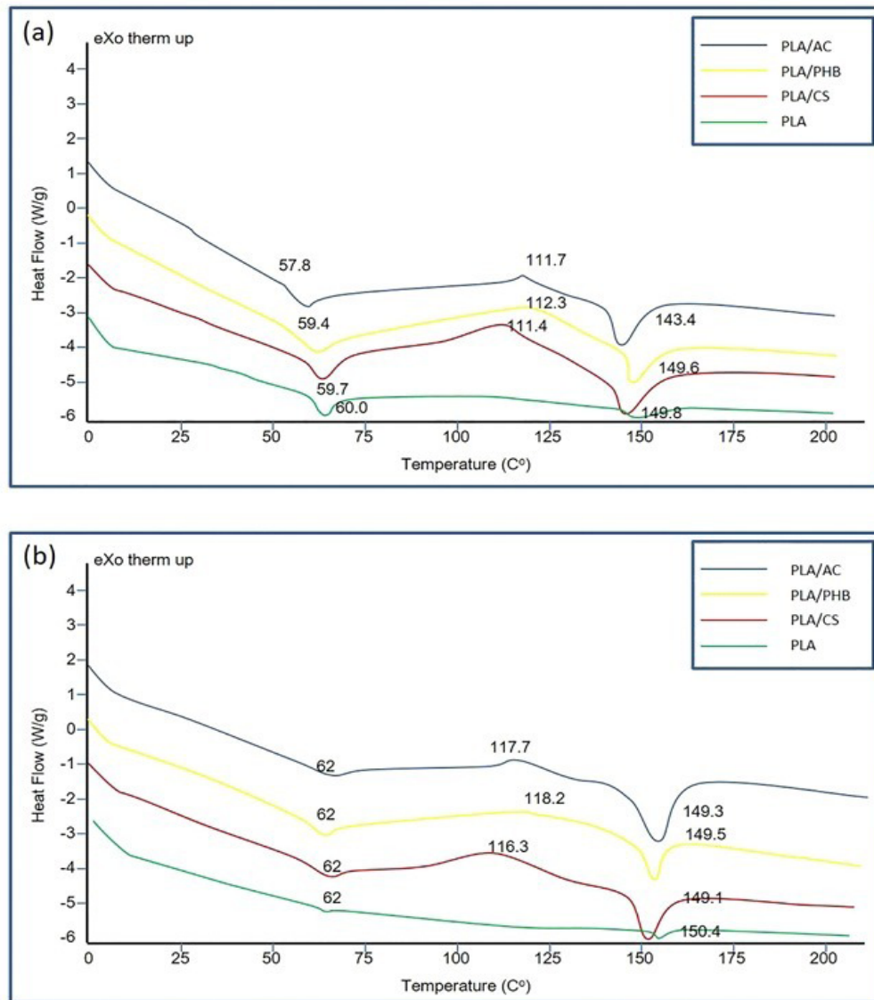
Fig. 3. DSC (a) first heating & (b) second heating of thermogravimetric for PLA and PLA biocomposites.
