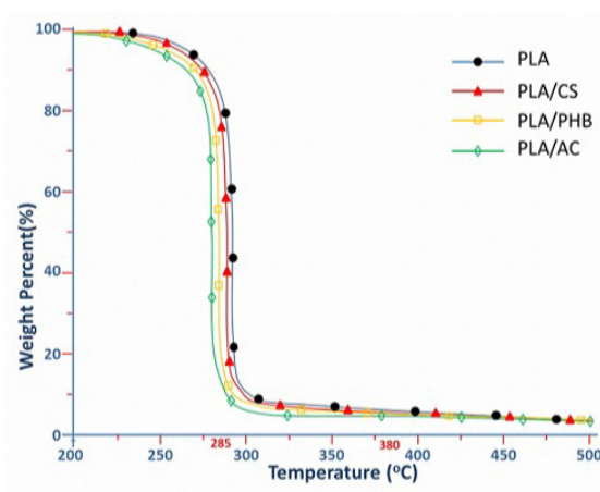
Fig. 2. TGA curves for PLA and PLA bio-composite samples.
