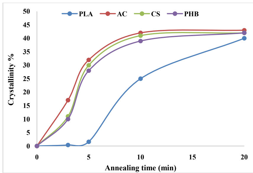
Fig. 4. Degree of crystallinity of PLA and PLA bio-composites with different annealing times.
