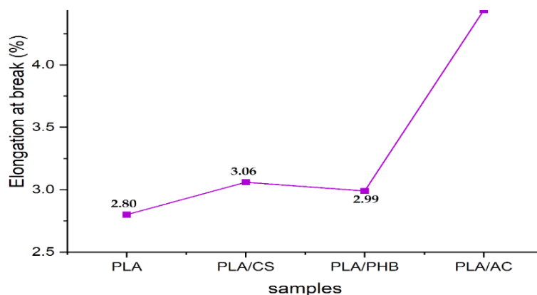
Fig. (1.c) E% for PLA and PLA Bio-composites .
