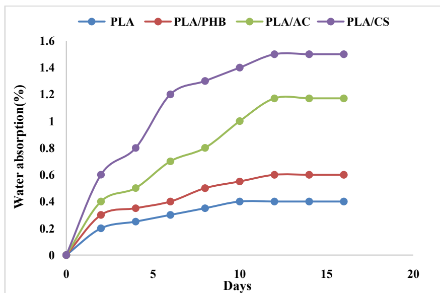
Fig. 5. Course of water uptake by PLA-films.
